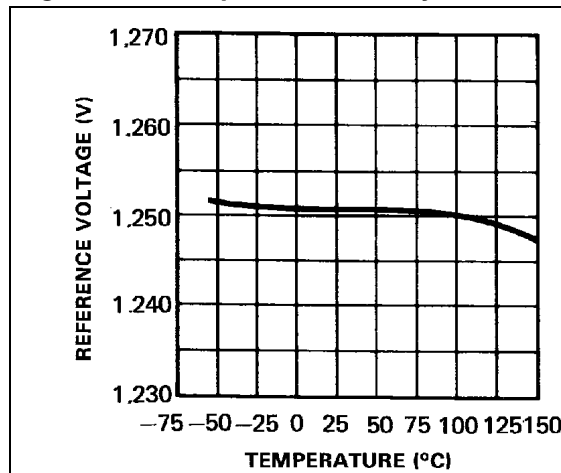
Figure 7. Temperature stability
